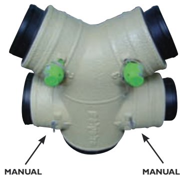
Fitting set up for 4 outlets (2x motorized/ 2x manual)
